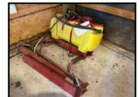
Scorpion 3 pt. 25 gallon sprayer 12 volt w/10' boom
